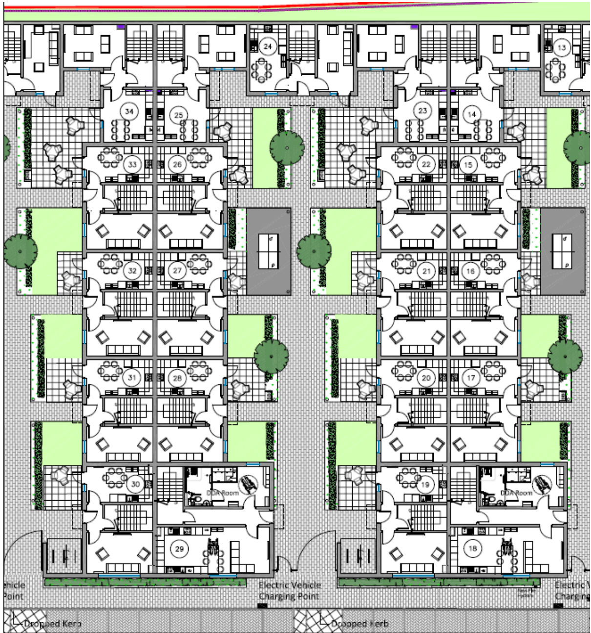
Typical courtyard layout
