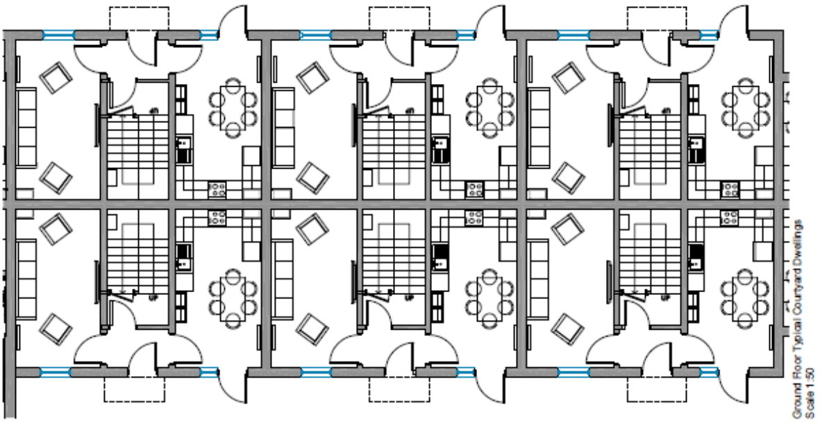
Typical courtyard dwellings- ground and first floor
